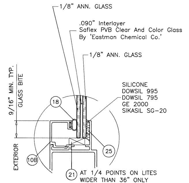
GLASS TYPE 'C' 5/16" OVERALL LAM. GLASS
